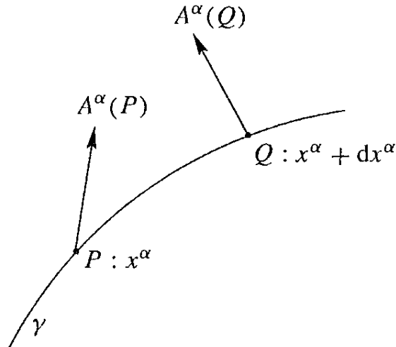
Figure 1.2 Differentiation of a tensor.
