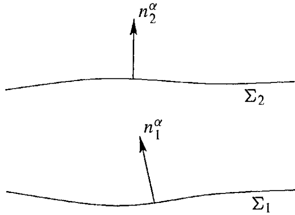
Figure 3.4 Two spacelike surfaces and their normal vectors.
