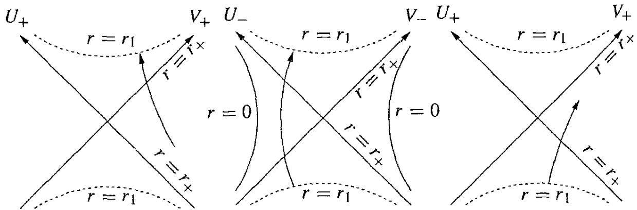
Figure 5.8 Kruskal patches for the Reissner–Nordström spacetime.
