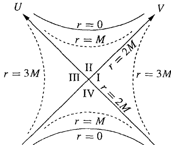
Figure 5.2 Kruskal diagram.
