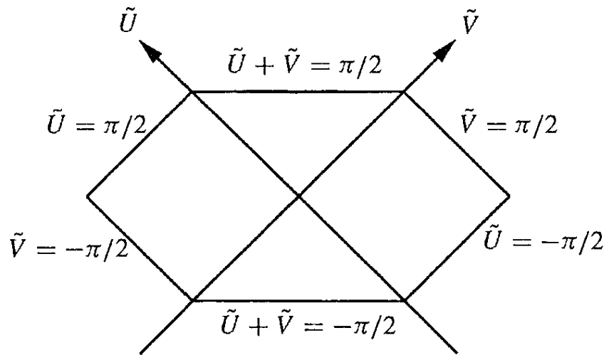
Figure 5.4 Compactified coordinates for the Schwarzschild spacetime.
