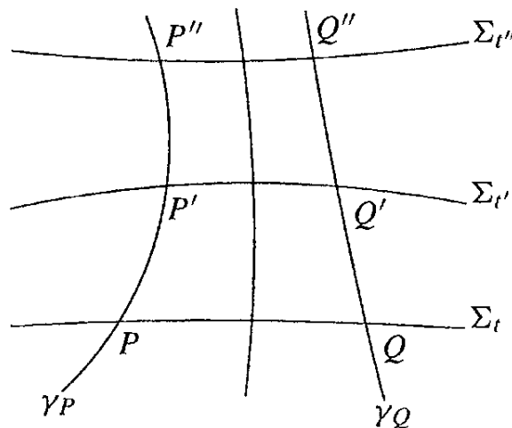
Figure 4.2 Foliation of spacetime by spacelike hypersurfaces.
