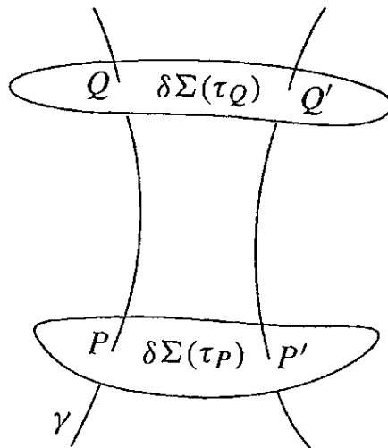
Figure 2.6 Congruence's cross section about a reference geodesic.
