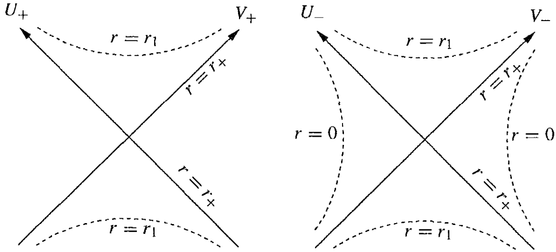
Figure 5.13 Kruskal patches for the Kerr spacetime.
