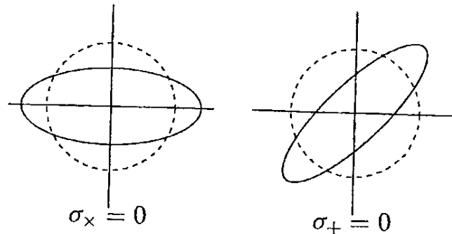
Figure 2.2 Effect of the shear tensor.
