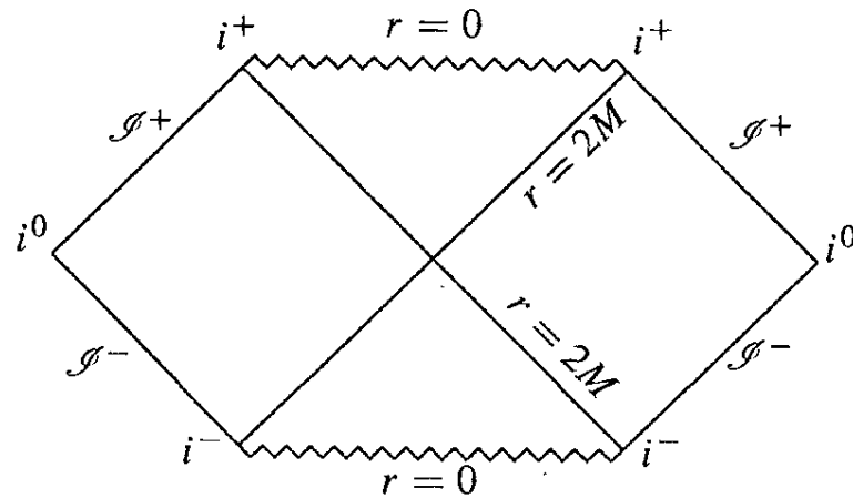
Figure 5.5 Penrose–Carter diagram of the Schwarzschild spacetime.
