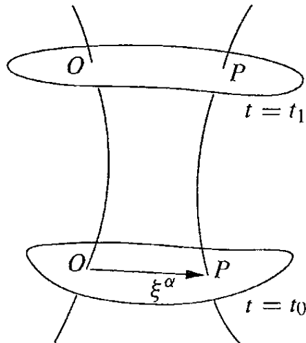
Figure 2.1 Two-dimensional deformable medium.
