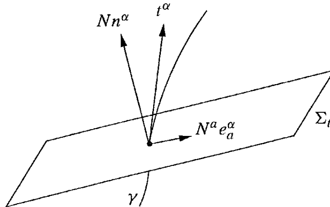
Figure 4.3 Decomposition of t^\alpha into lapse and shift.
