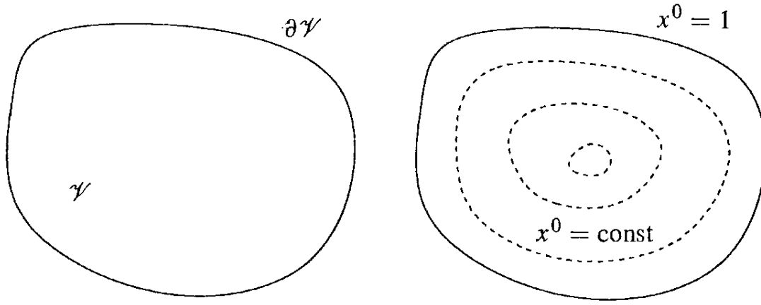
Figure 3.3 Proof of the Gauss-Stokes theorem.
