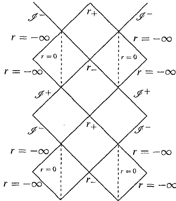
Figure 5.14 Penrose–Carter diagram of the Kerr spacetime.
