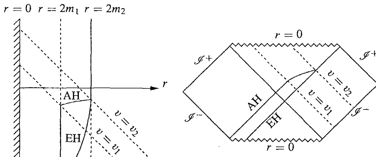
Figure 5.7 Black hole irradiated with ingoing null dust.
