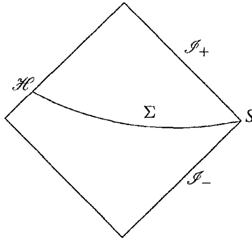
Figure 5.17 A spacelike hypersurface in a black-hole spacetime.
