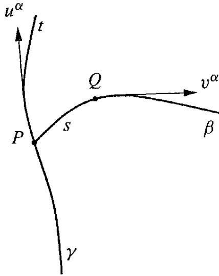
Figure 1.4 Geometric construction of the Fermi normal coordinates.
