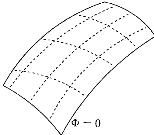
Figure 3.1 A three-dimensional hypersurface in spacetime.
