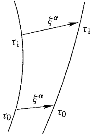
Figure 2.3 Deviation vector between two neighbouring members of a congruence.
