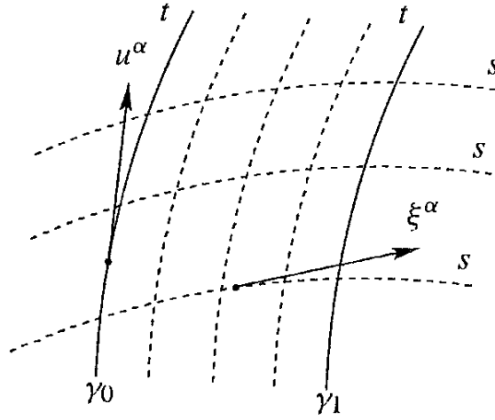
Figure 1.3 Deviation vector between two neighbouring geodesics.
