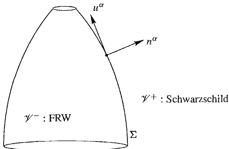
Figure 3.6 The Oppenheimer–Snyder spacetime.
