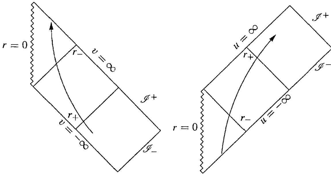
Figure 5.11 Eddington–Finkelstein patches for the Reissner–Nordström spacetime.
