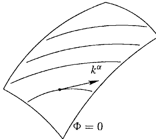
Figure 3.2 A null hypersurface and its generators.
