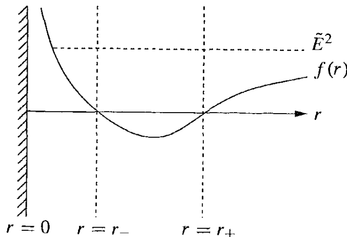
Figure 5.10 Effective potential for radial motion in Reissner–Nordström spacetime.
