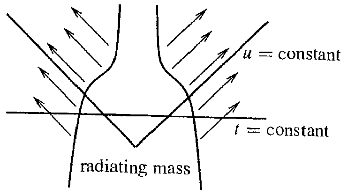
Figure 4.5 A radiating spacetime.
