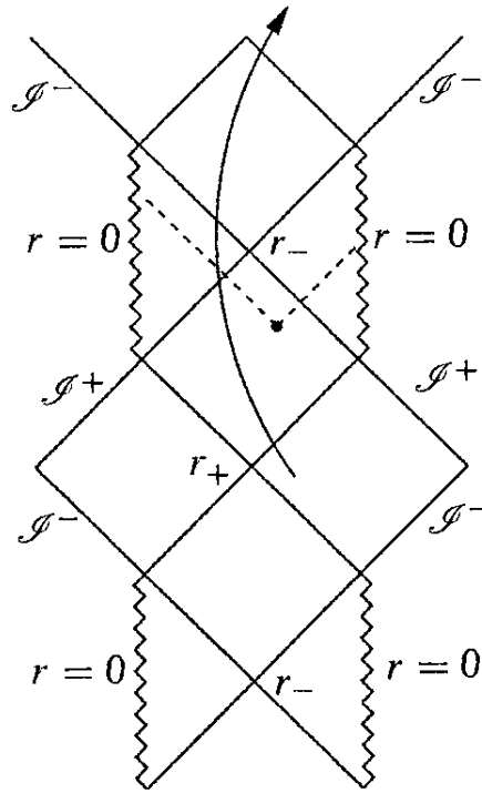
Figure 5.9 Penrose–Carter diagram of the Reissner–Nordström spacetime.
